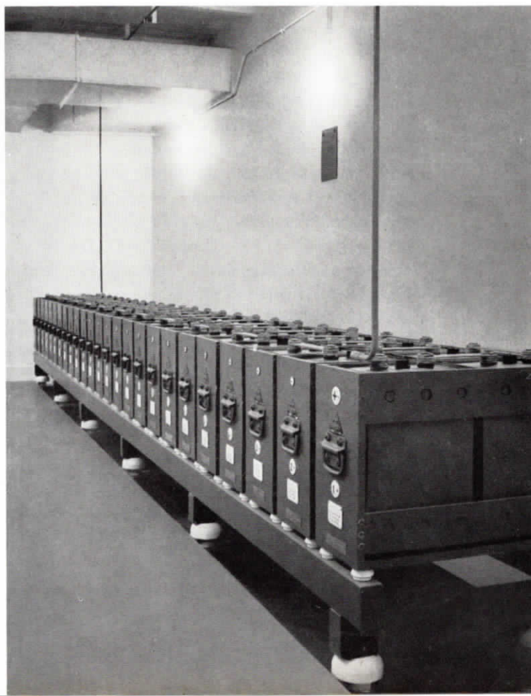
NICKEL-CADMIUM-BATTERIE 60 V 840 Ah
